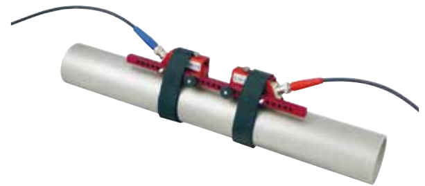
The DUC Ultrasonic Flow Meter is one of KOBOLD's many flow meters used in ESG, for flow and heat transfer measurement.
